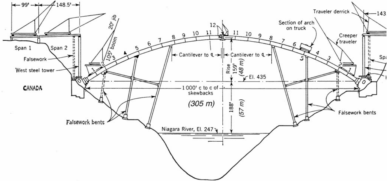
Figure 45.5 Lewiston-Queenston arch bridge near Niagara Falls, New York. Crawler cranes erect steelwork for spans 1 and 6 and erect material derricks thereon. These derricks erect traveler derricks, which move forward and erect supporting falsework and spans 2, 5, and 4. Traveler derricks erect arch-rib sections 1 and 2 and supporting falsework at each skewback, then set up creeper derricks, which erect arches to midspan.
