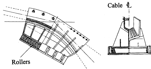
Side elevation
