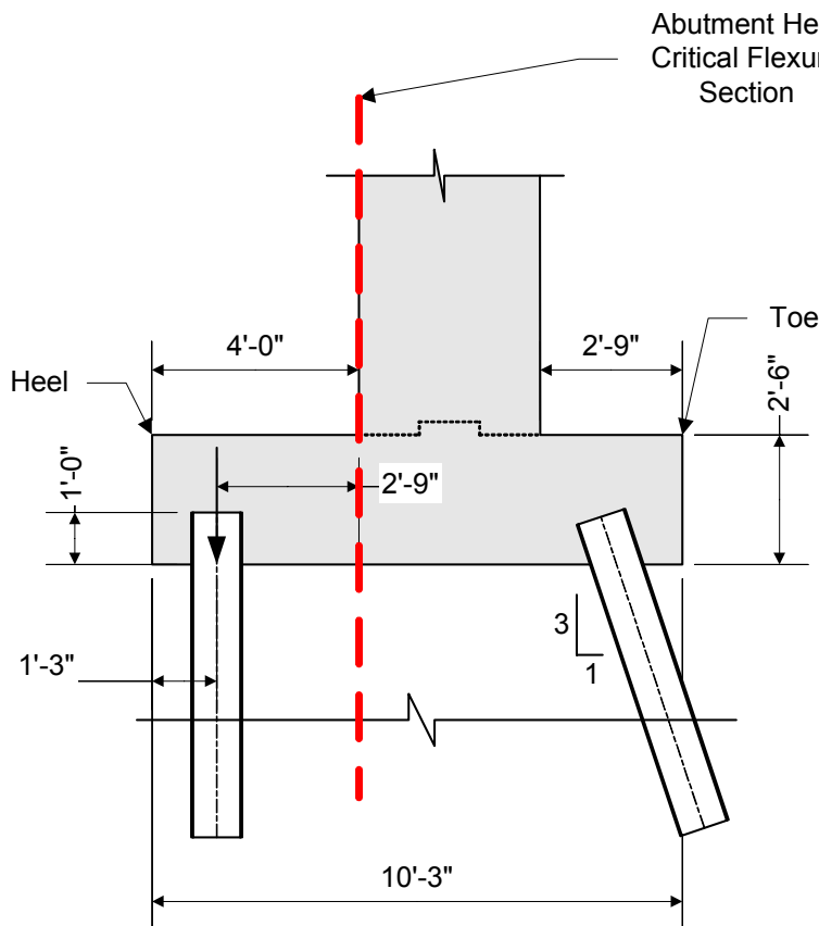
Figure 7-20 Abutment Heel Critical Flexure Section
