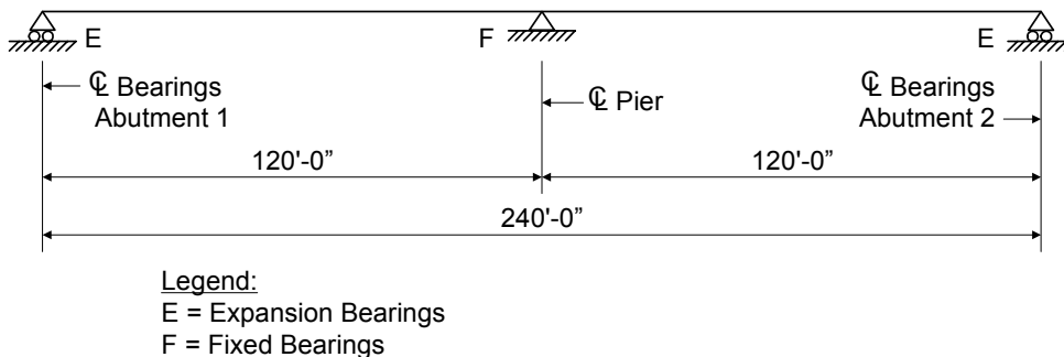
Figure 1-1 Span Arrangement
