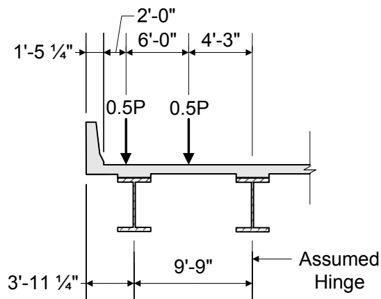
Figure 3-5 Lever Rule
