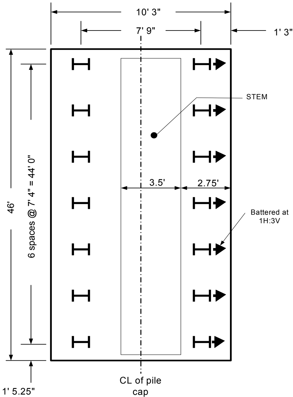
Figure P-16 Final Pile Cap Layout
