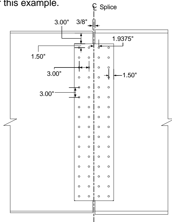
Figure 4-8 Web Splice
