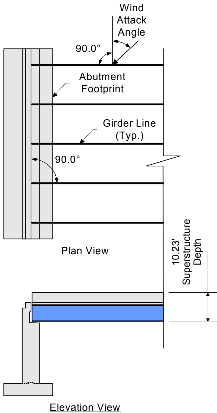
Figure 7-3 Application of Superstructure Wind Load on Abutment
