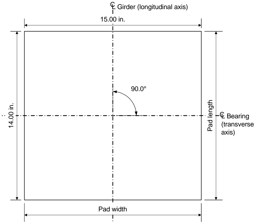
Figure 6-1 Bearing Pad Plan View
