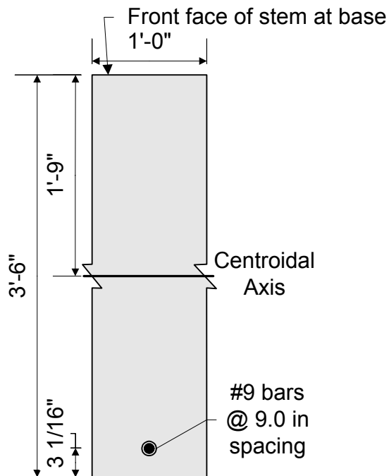
Figure 7-13 Abutment stem Cracking Moment Dimensions
