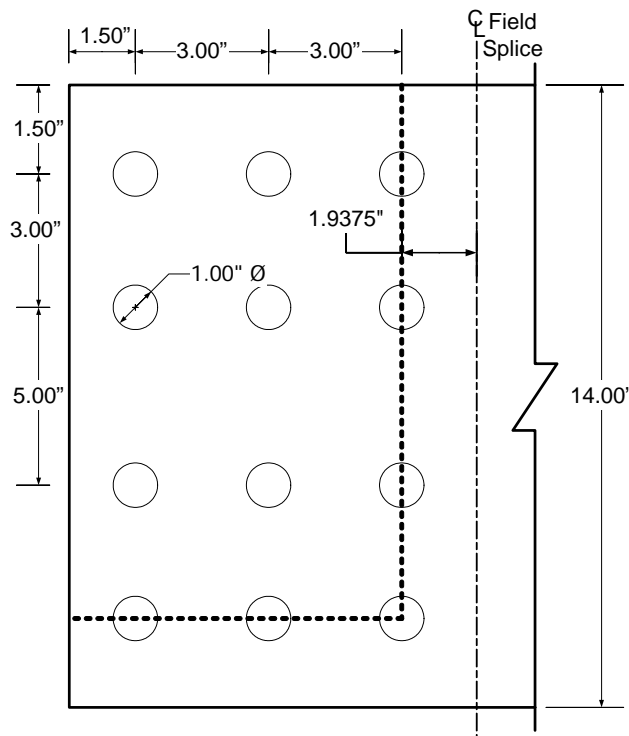
Figure 4-4 Outside Splice Plate - Failure Mode 1
