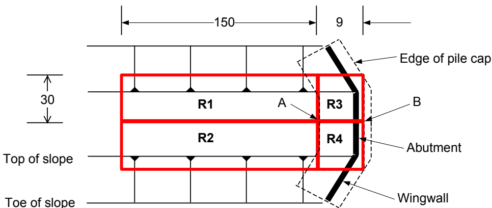
Figure P-15 Plan View of Approach Embankment
