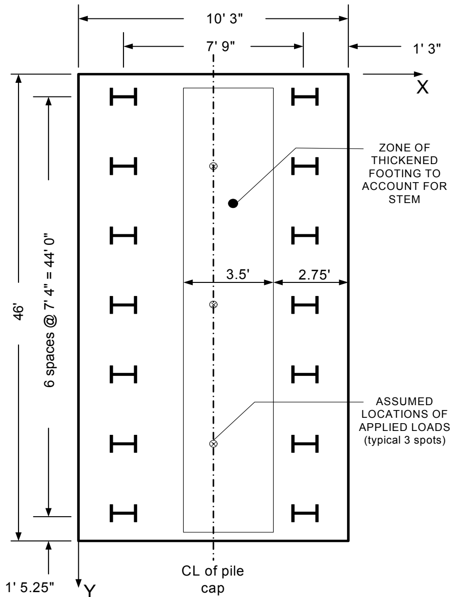
Figure P-12 Location and Thickness of Stem
