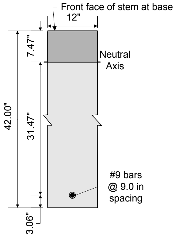
Figure 7-14 Abutment Stem Crack Control Check
