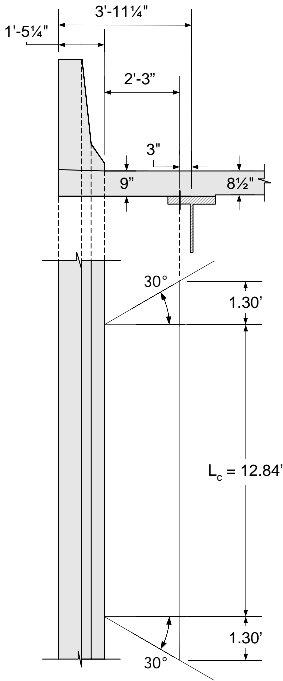
Figure 2-11 Assumed Distribution of Collision Moment Load in the Overhang
