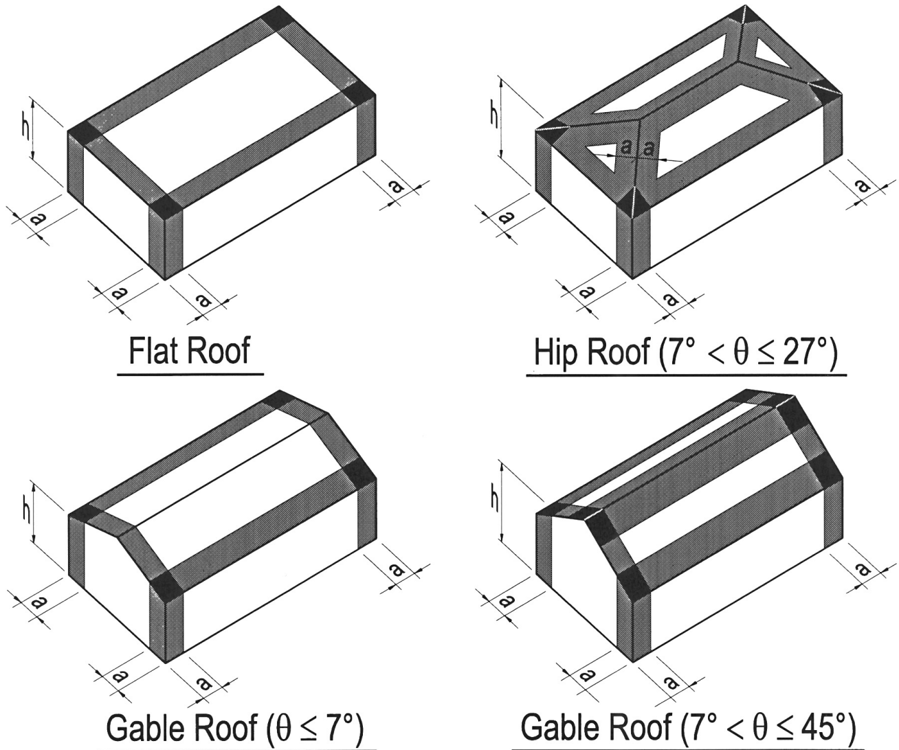
FIGURE 1609.6.2.2 COMPONENT AND CLADDING PRESSURE
