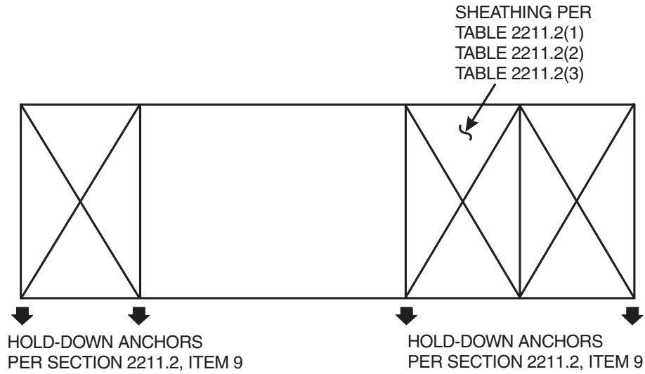
TYPE 1 SHEAR WALL
