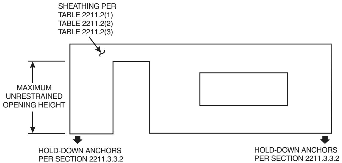
TYPE II SHEAR WALL
